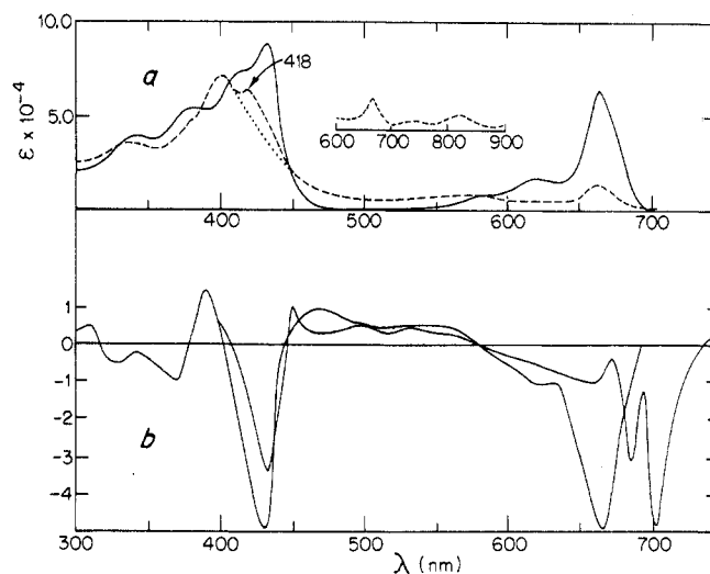
Figure 4. (a) Optical absorption spectra of Chl a (—) and Chl a^{\cdot+} (---) in methylene dichloride. A small amount of decomposition product ( \lambda_{\max} 418 nm) appears during the electrochemical oxidation. (b) The optical difference spectrum 32 of Chl a and Chl a^{\cdot+} (calculated from a) and the difference spectrum of photosynthesizing chloroplasts. The observation of an absorption band in the near infrared of the chlorophyll \pi cation radical (---) suggested that such an absorption should be observed in the near-infrared difference spectrum of photosynthesizing chloroplasts; such an observation 32 has been recently made.
